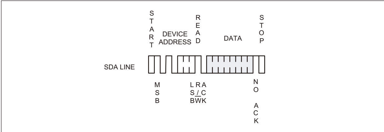
► Figure 8: Random Read
